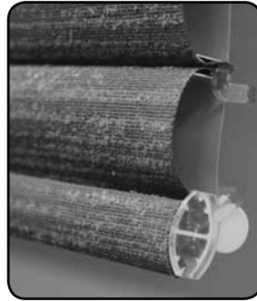
Fabric Wrapped Bottom Rail
